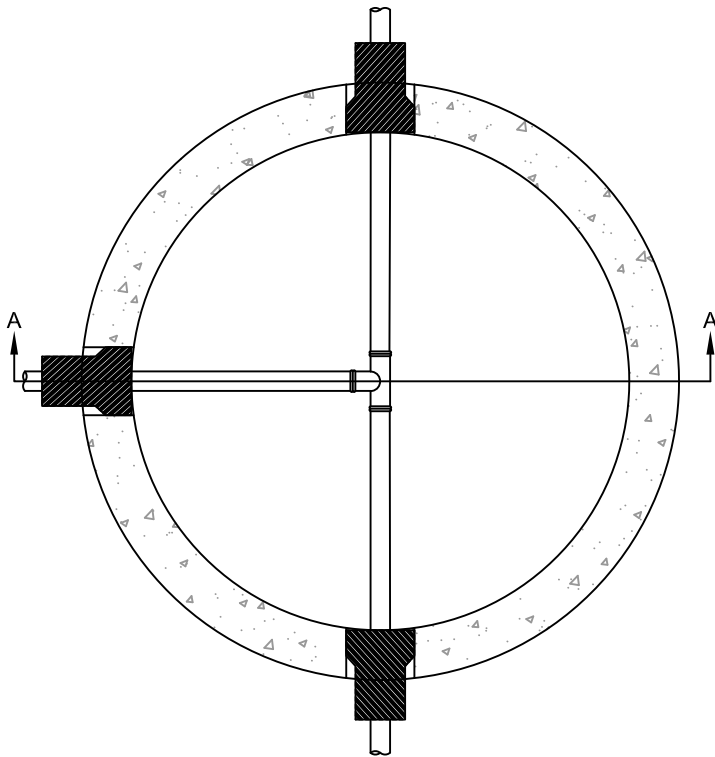
3-WAY JUNCTION MANHOLE
