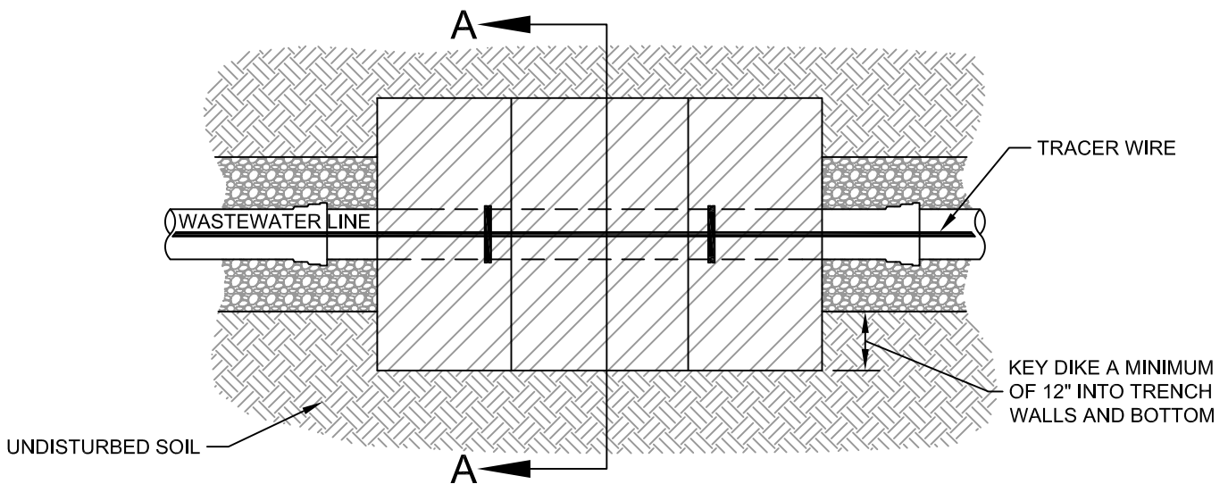
PLAN
