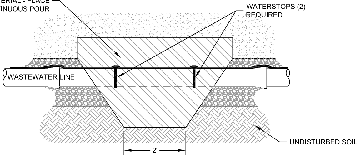
PROFILE
